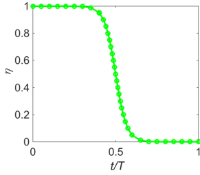
Fig. 3. Dynamic changing trajectory of \eta with \alpha = 0.5 and \Gamma = 30 .
